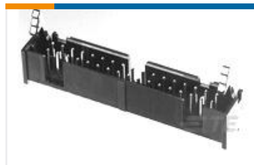
TE Part #1761606-9 IDC LOW PRO HDR 26P VERT LG LA
