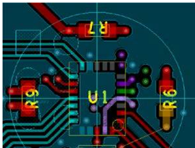
Figure 10. Placement of Heating Resistors
