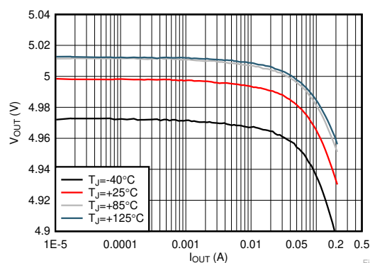
Load Regulation
