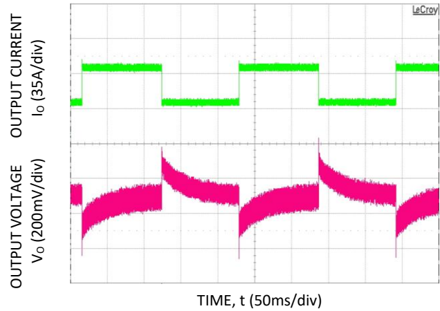
Figure 8. 12V transient response for 50 to 100% step load, Vin: -48V DC , slew rate 1A/μs.
