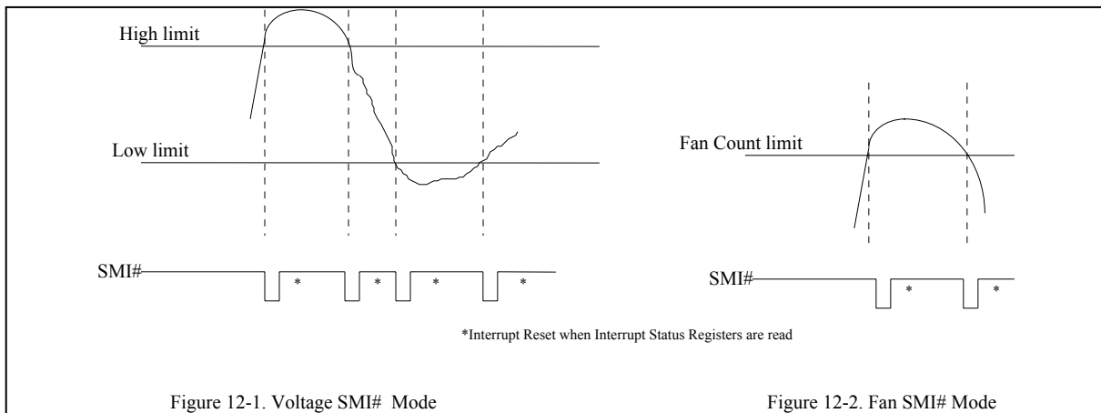
Figure 12-1. Voltage SMI# Mode
