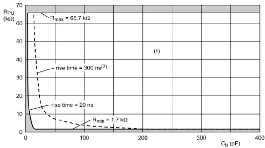
Figure 8. Bus Requirements for 3.3V Systems
