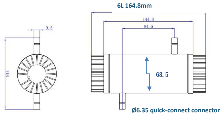
Fig.2 Outline Dimensions
