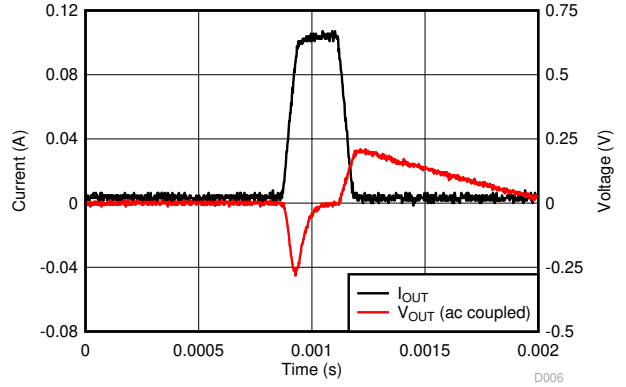
V_{OUT} = 5\ \text{V} , C_{IN} = 1\ \mu\text{F} , C_{OUT} = 1\ \mu\text{F} , I_{OUT} = 1\ \text{mA} \rightarrow 100\ \text{mA} → 1\ \text{mA} , Slew rate = 1\ \text{mA}/\mu\text{s}
