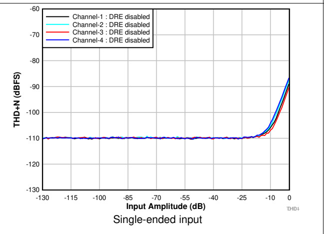
Figure 8. THD+N vs Input Amplitude With DRE Disabled
