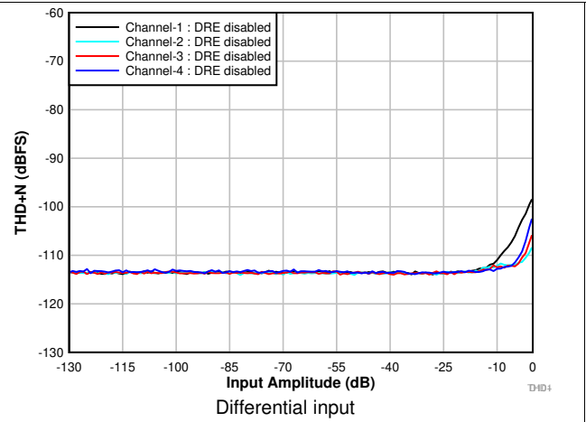
Figure 6. THD+N vs Input Amplitude With DRE Disabled
