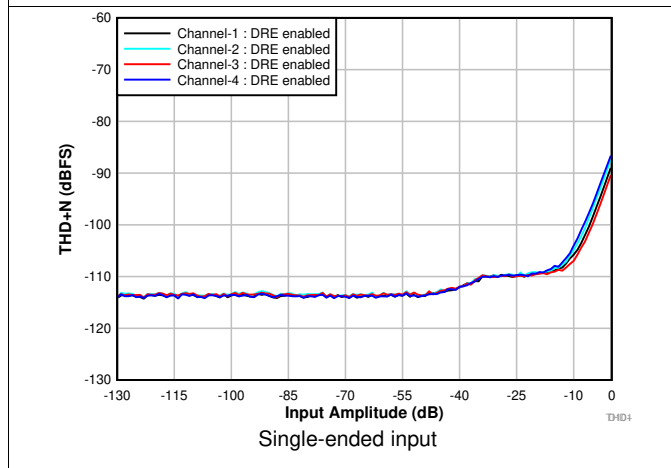
Figure 7. THD+N vs Input Amplitude With DRE Enabled
