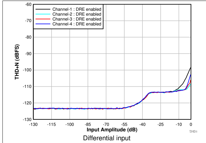
Figure 5. THD+N vs Input Amplitude With DRE Enabled
