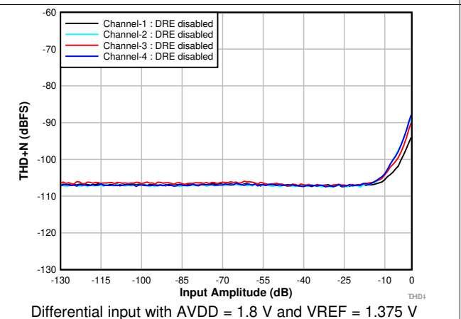
Figure 10. THD+N vs Input Amplitude With DRE Disabled
