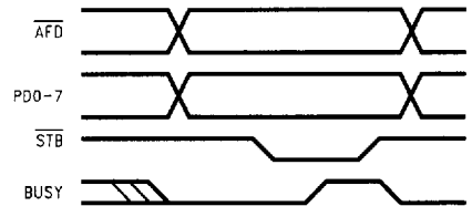
FIGURE 7-6. ECP Forward Write Cycle
