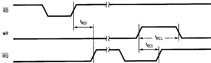
FIGURE 11-24. \overline{IR\overline{Q}} Release Delay
