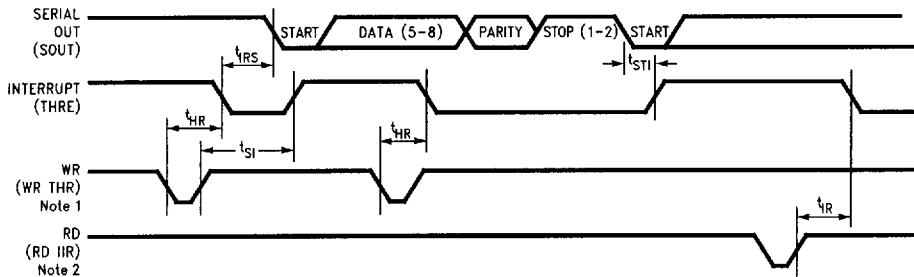
FIGURE 11-6. Transmitter Timing
