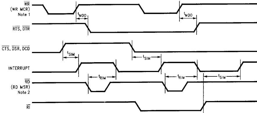
FIGURE 11-11. MODEM Control Timing
