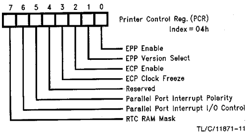
FIGURE 2-1. PC87323 Configuration Registers
