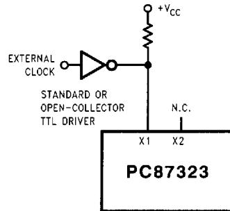
FIGURE 9-12. External Clock Connection
