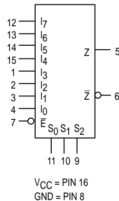
LOGIC SYMBOL
