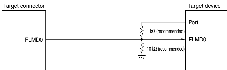
Figure 28-3. Connection of FLMD0 Pin for Self Programming by Means of On-Chip Debugging
