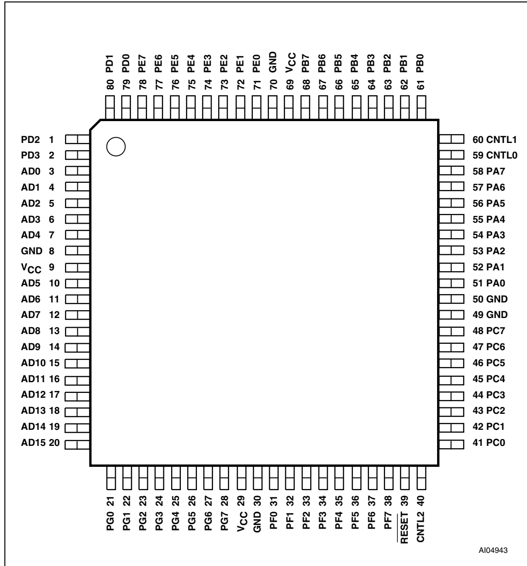
Figure 2. LQFP connections
