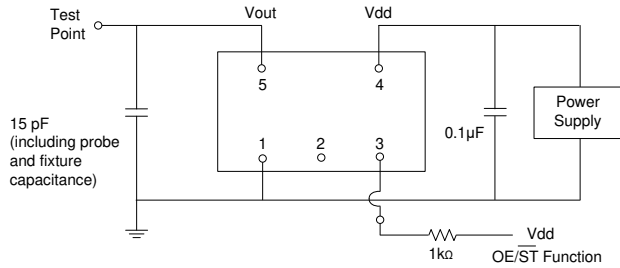
Figure 2. Test Circuit [6]
