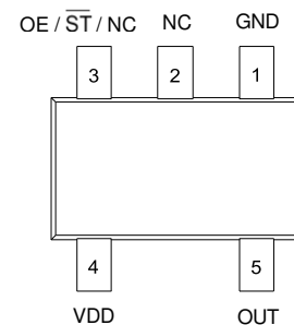
Figure 1. Pin Assignments
