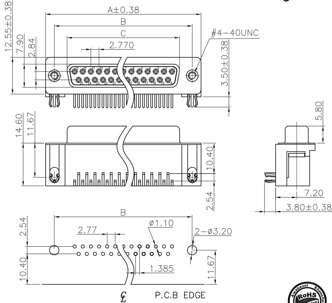
RECOMMENDED P.C.B LAYOUT TOLERANCE±0.05
