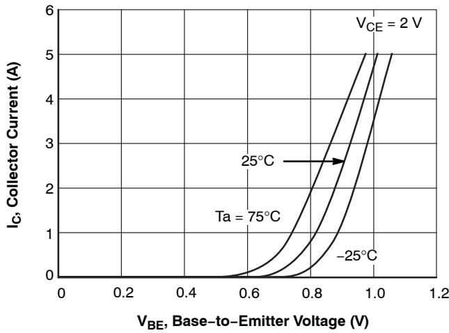
Figure 4. I_C - V_{BE}
