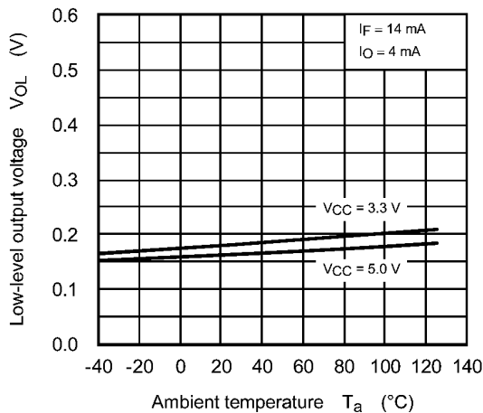
Fig. 12.2.3 V_{OL} - T_a
