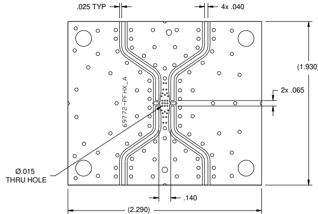
2dB - 5dB Test Board
