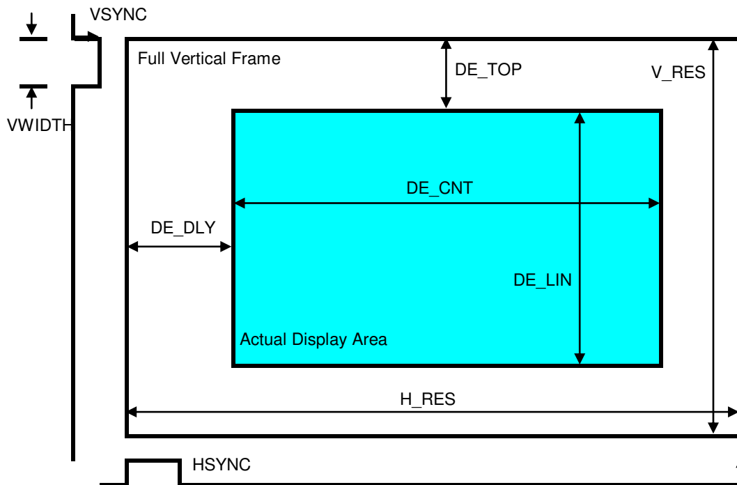
FIGURE 7. DE GENERATOR MEASUREMENTS
