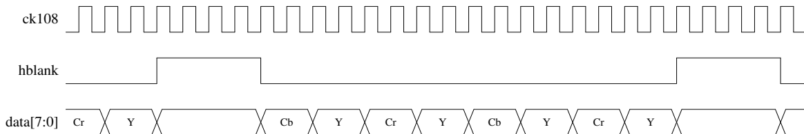
Horizontal Timing (54M)
