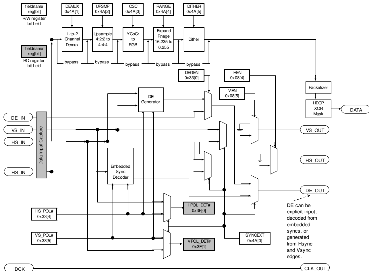
FIGURE 13. TRANSMITTER VIDEO DATA PROCESSING PATH
