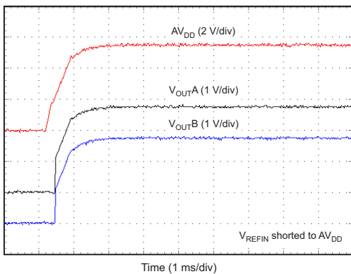
Figure 36. Power-On Glitch Reset to Mid-Scale
