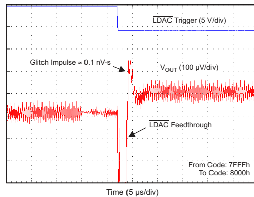
Figure 37. Glitch Impulse Rising Edge, 1-LSB Step
