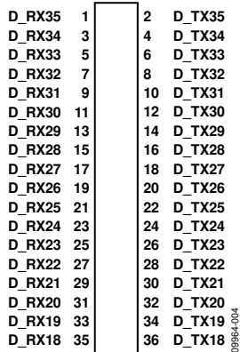
Figure 4. J5 Configuration
