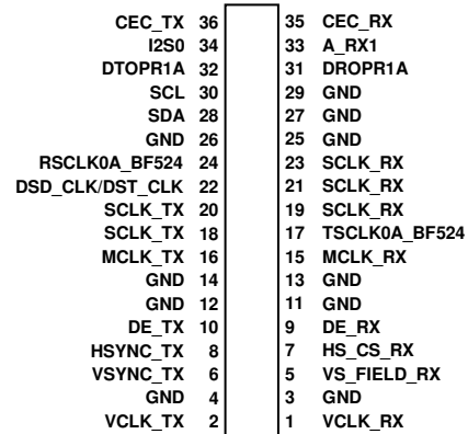
Figure 7. J4 Configuration
