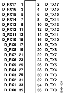
Figure 5. J6 Configuration
