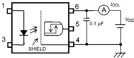
Fig. 12.1.3 IDDL Test Circuit
