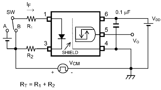
Fig. 12.1.7 Common-Mode Transient Immunity Test Circuit and Waveform
