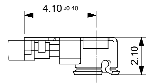
DETAIL B SCALE 8x CONNECTOR
