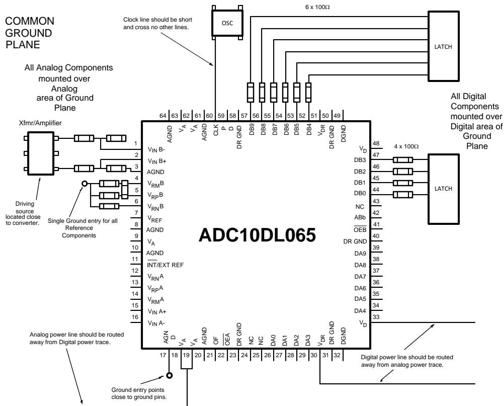
Figure 39. Example of a Suitable Layout
