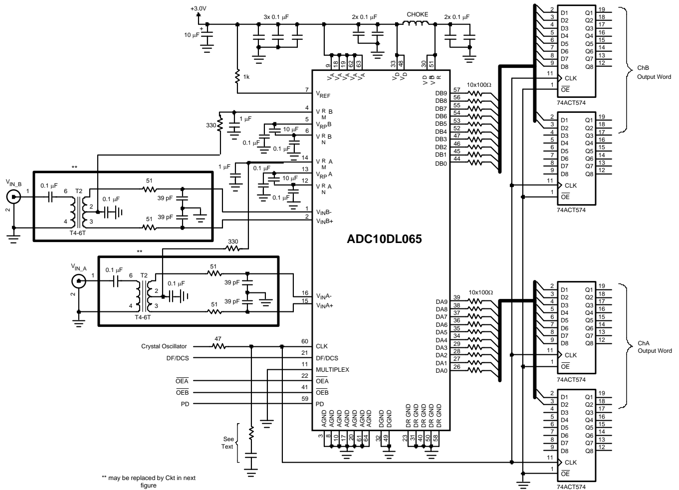
Figure 36. Application Circuit Using Transformer Drive Circuit, Parallel Mode
