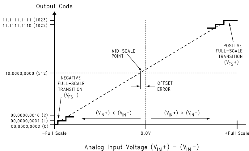
Figure 2. Transfer Characteristic
