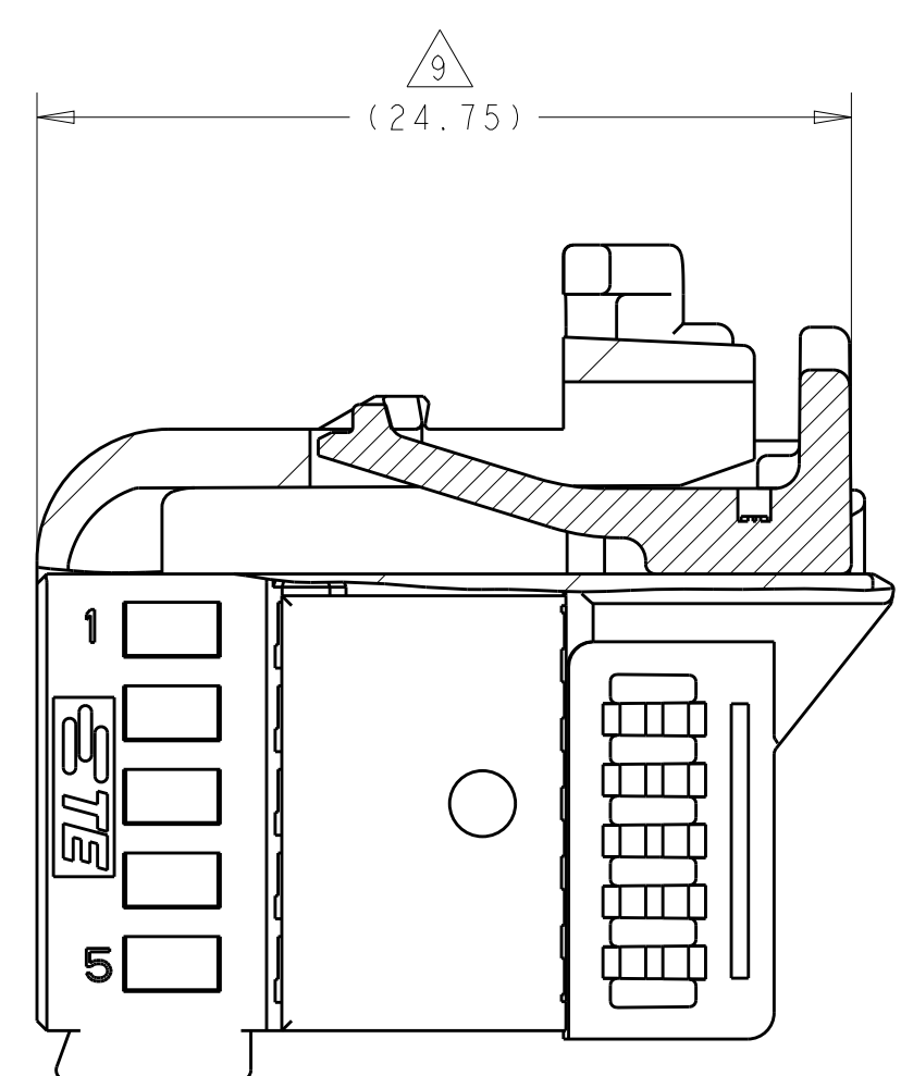
SECTION X - X CPA SHOWN IN LOCKED POSITION
