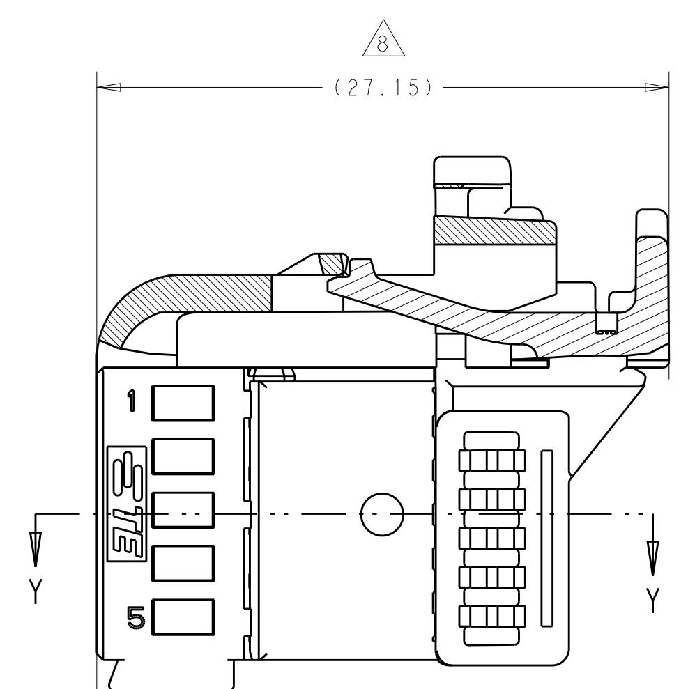
SECTION X - X CPA SHOWN IN PRE-LOCKED POSITION
