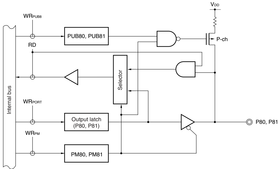
Figure 4-16. Block Diagram of P80 and P81
