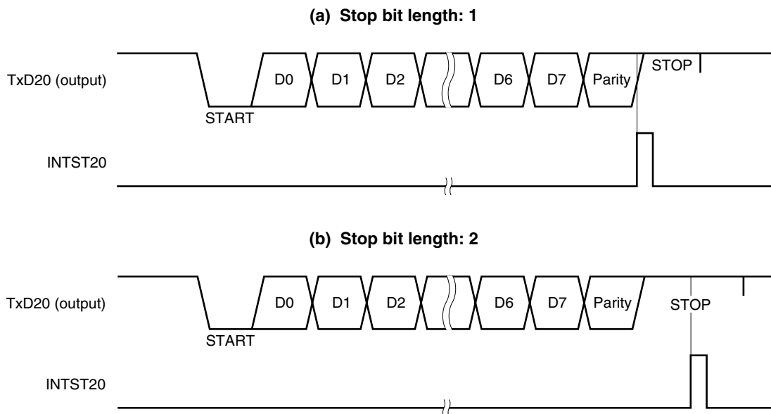
Figure 12-8. Asynchronous Serial Interface Transmission Completion Interrupt Timing
