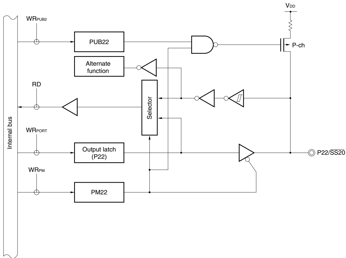
Figure 4-7. Block Diagram of P22
