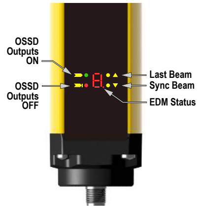
Figure 2. Status Indicators—Receiver
