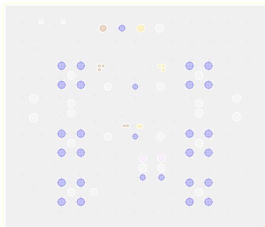
Figure 7. EVAL-ADG5401FEBZ, Layer 2
