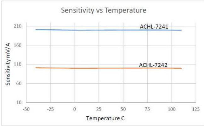
Figure 1: Sensitivity vs. Temperature
