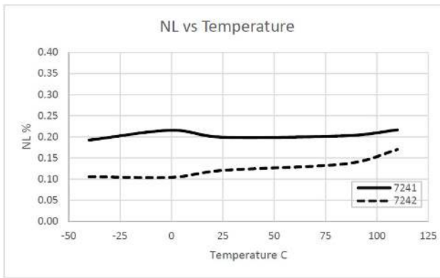
Figure 5: Nonlinearity vs. Temperature
