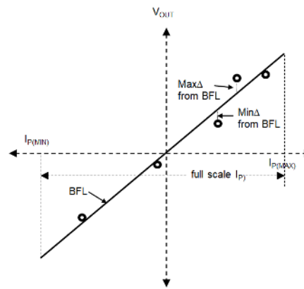
Figure 14: Nonlinearity Calculation
