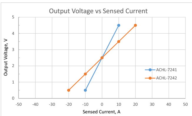
Figure 7: Output Voltage vs. Sensed Current
