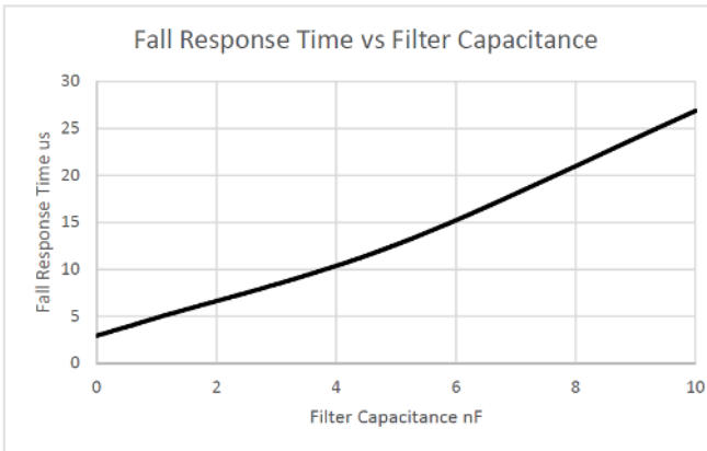
Figure 11: Fall Response Time vs. External Filter
