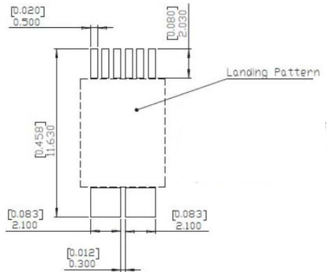
Figure 16: Land Pattern for 8-mm Creepage
