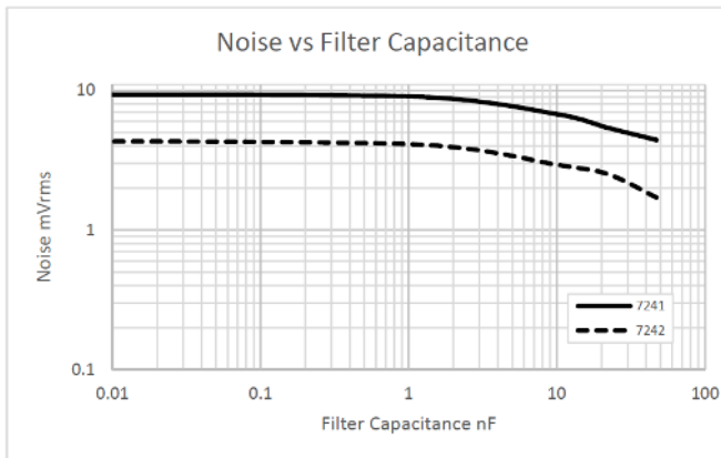
Figure 13: Output Noise vs. External Filter
