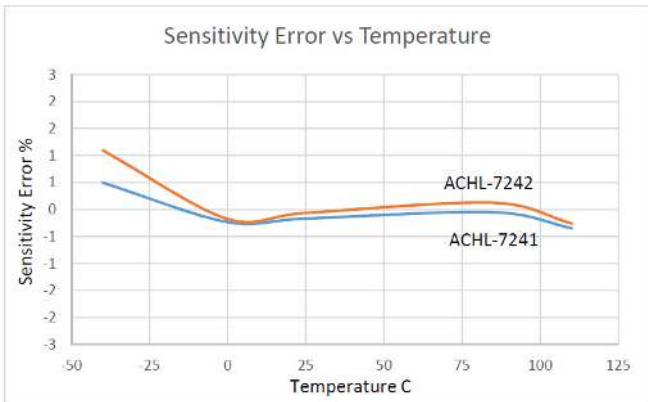
Figure 3: Sensitivity Error vs. Temperature
