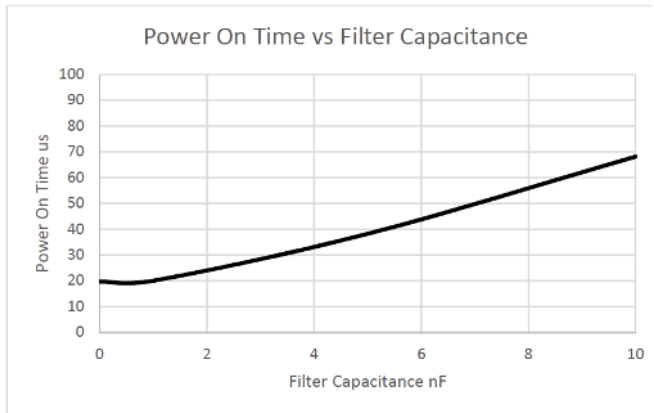
Figure 8: Power-On Time vs. External Filter
