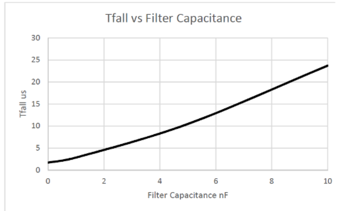
Figure 12: Tfall vs. External Filter
