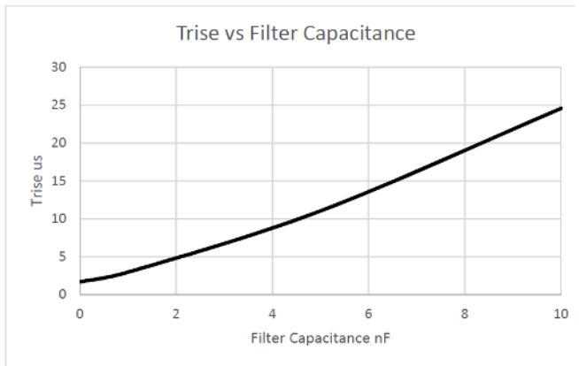
Figure 10: Rise Time vs. External Filter
