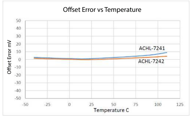
Figure 2: Offset Error vs. Temperature
