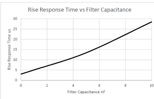
Figure 9: Rise Response Time vs. External Filter
