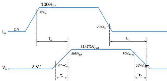
Figure 15: Rise/Fall Times and Rise/Fall Response Times
