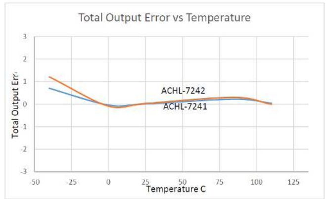
Figure 4: Total Output Error vs. Temperature
