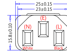
ME-302 (IEC 60320, C13) (Dimensions of Connector Face)
