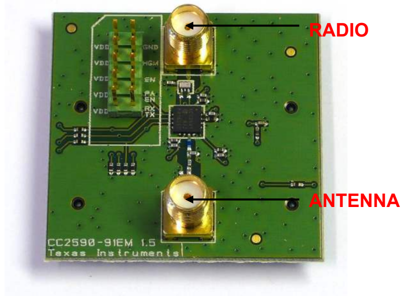
Figure 1 - CC2591EM
