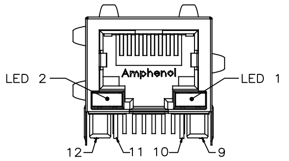
TYPICAL FOR SINGLE & MULTI-PORT
