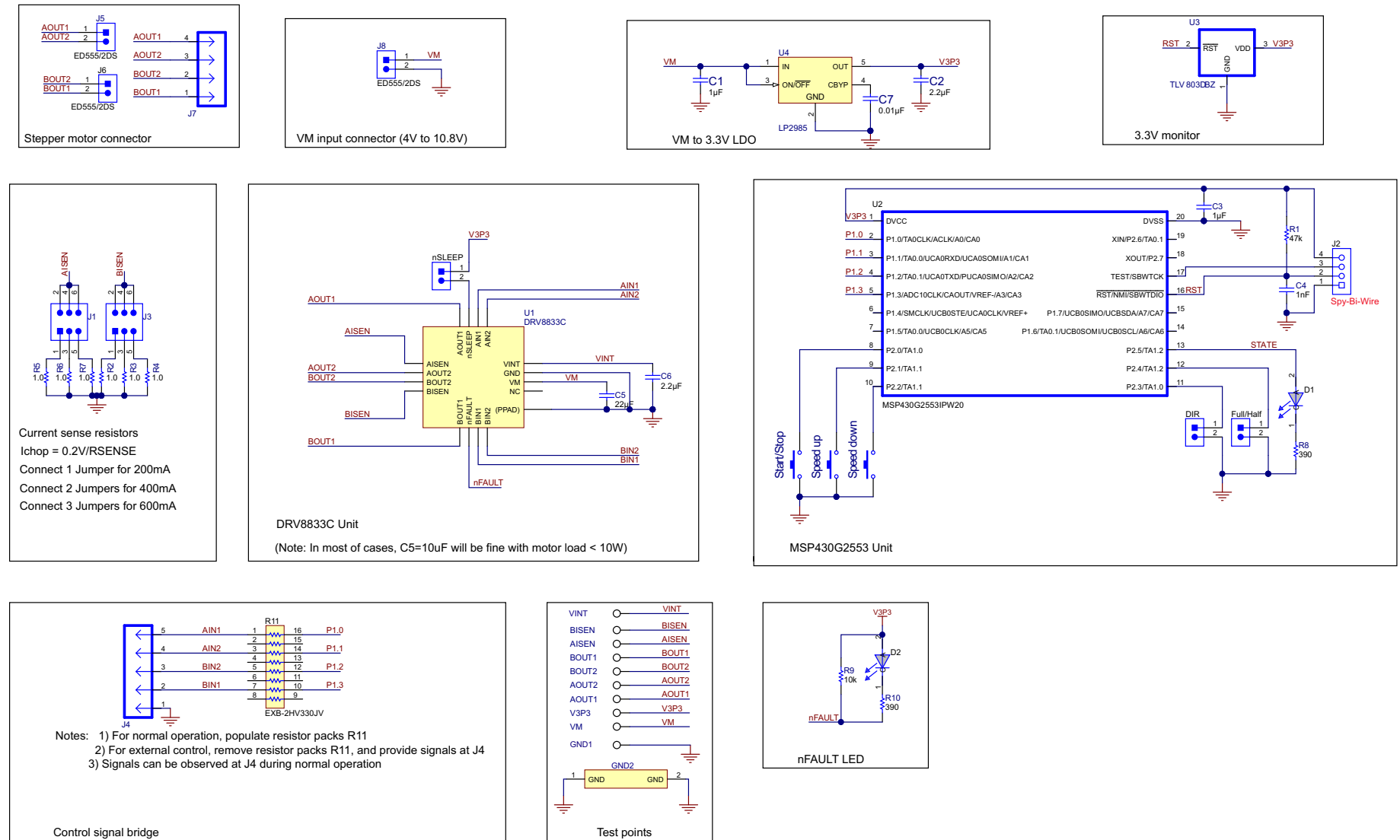
Figure 5. EVM Schematic
