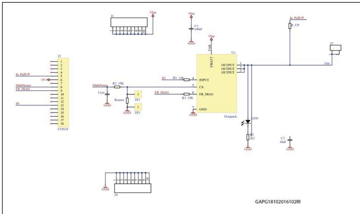
Figure 1. EV-VN7004CLH schematic
