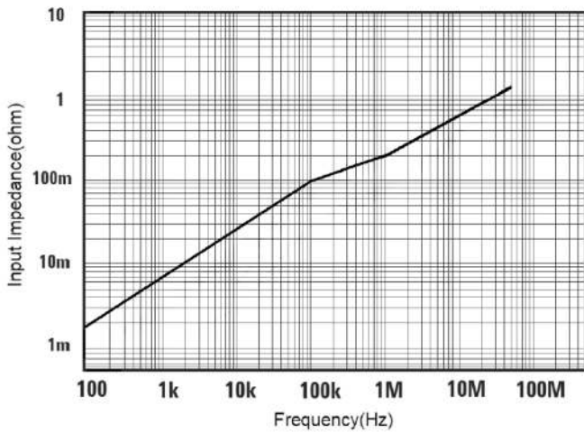
T3CP50-50 Insertion Impedance
