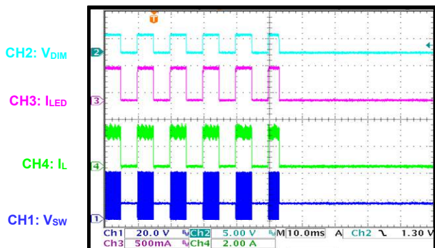
PWM Dimming Off
