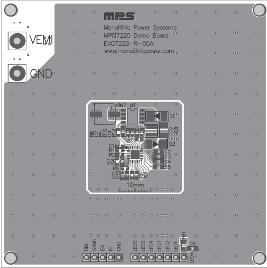
Figure 2: Top Silk Layer and Top Layer
