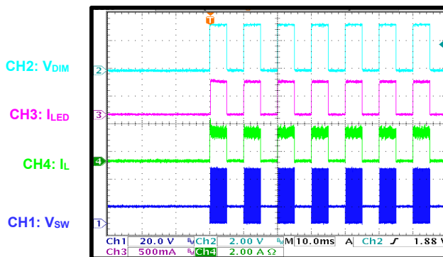
PWM Dimming On
