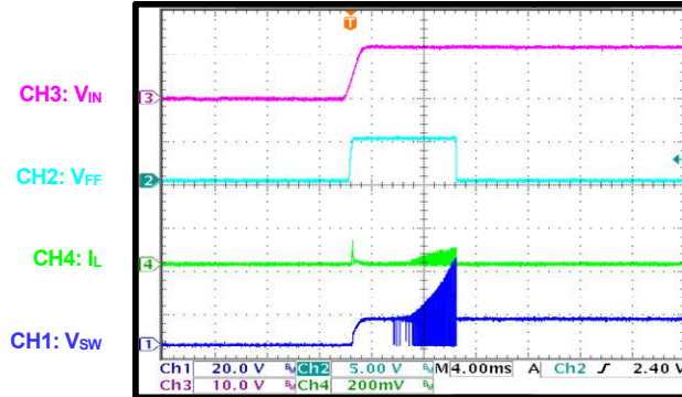
All 6 Strings LED Open Power On
