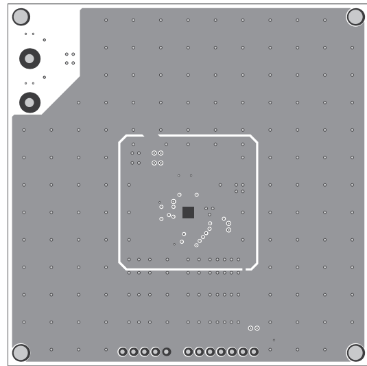
Figure 3: Mid-Layer 1
