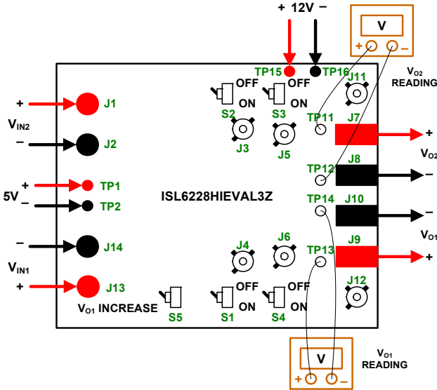
FIGURE 1. TEST SET-UP
