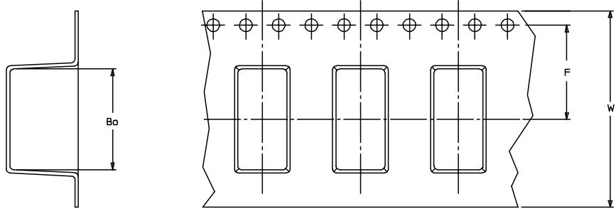
EMBOSED CARRIER TAPE TYPE 'A'
