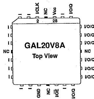
Chip Carrier
