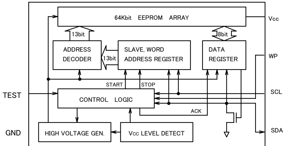
Figure 2. Block Diagram
