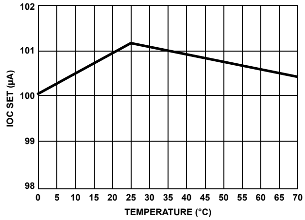
FIGURE 12. OCSET CURRENT vs TEMPERATURE
