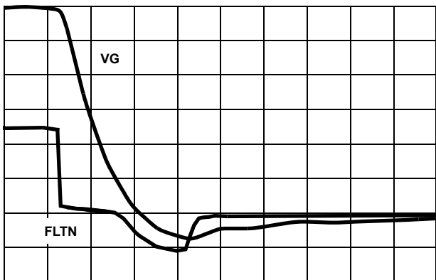
VOLTAGE (2V/DIV) TIME (1 \mu s/DIV) FLTN = OPEN
